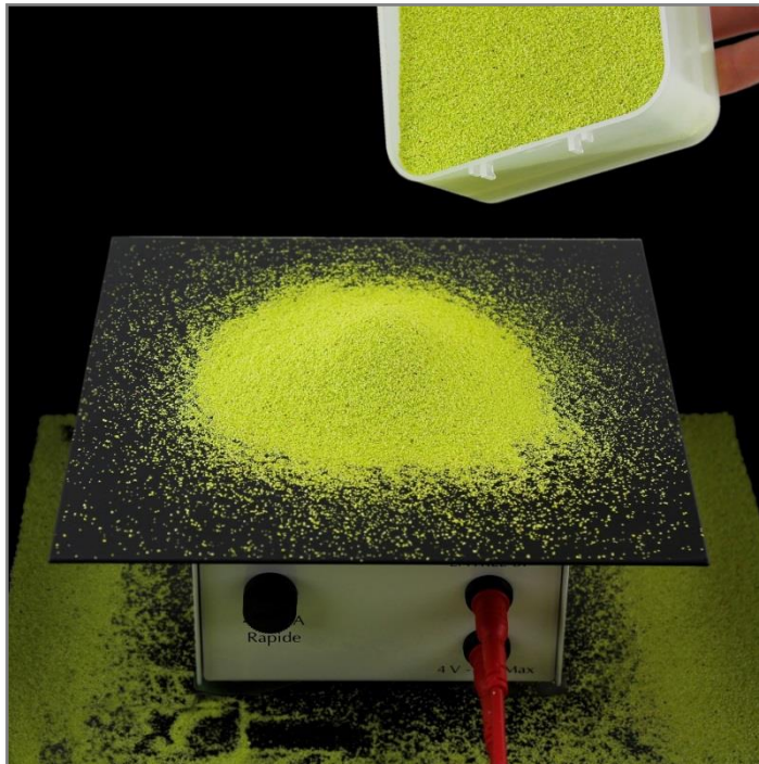
CHLADNI experiment on Melde vibrator
