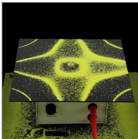
CHLADNI figures on Melde vibrator with the square slab
