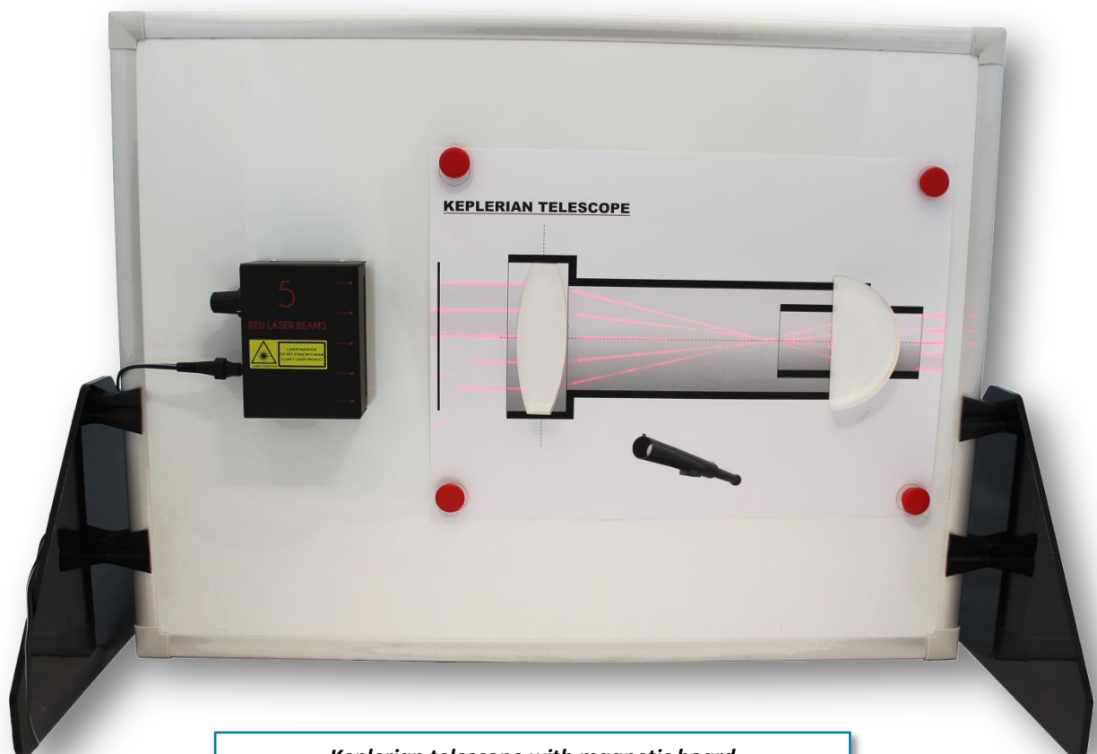
Keplerian telescope with magnetic board
