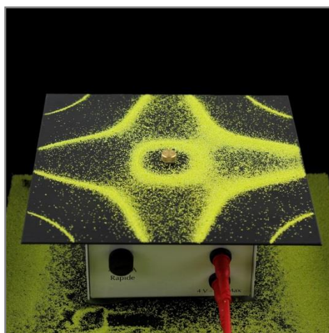
CHLADNI experiment with square and violin slabs
